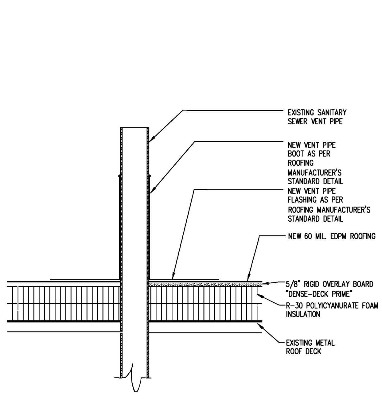
1 SANITARY SEWER VENT DETAIL A2 1.5"=1'-0"
