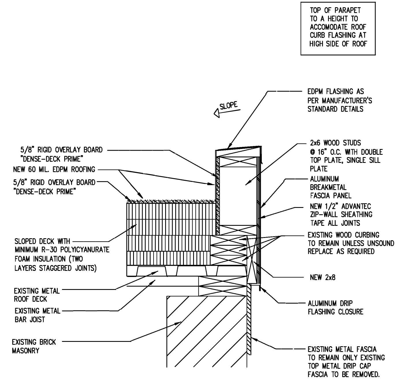
3 NON BEARING WALL CAP DETAIL A2 1.5"=1'-0"
