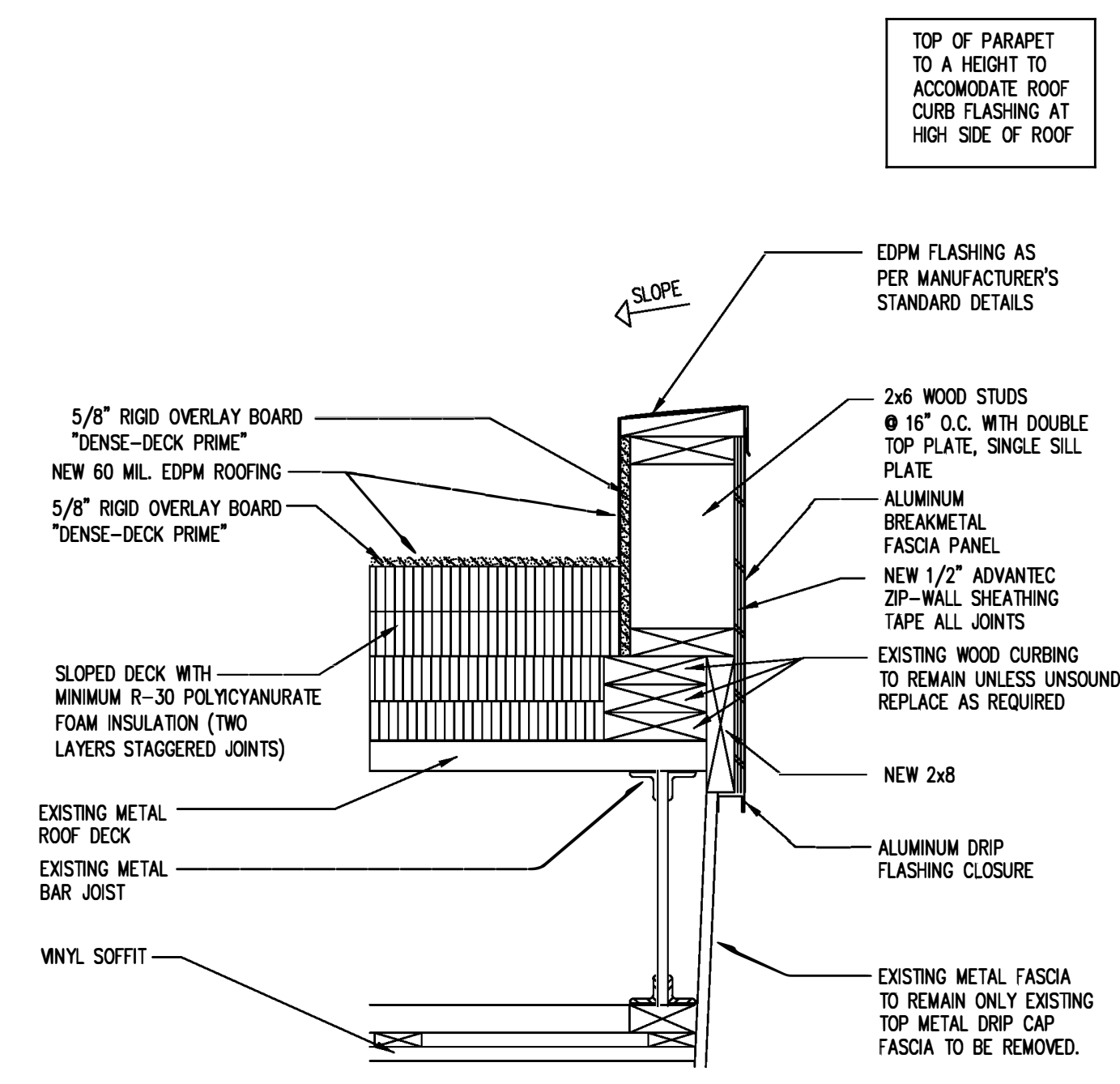
5 WALL CAP DETAIL A2 1.5"=1'-0"
