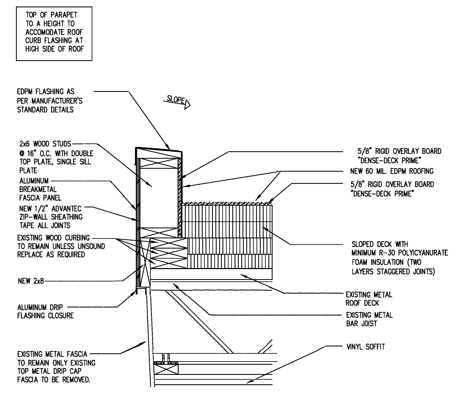
6 WALL CAP DETAIL A2 1.5"=1'-0"
