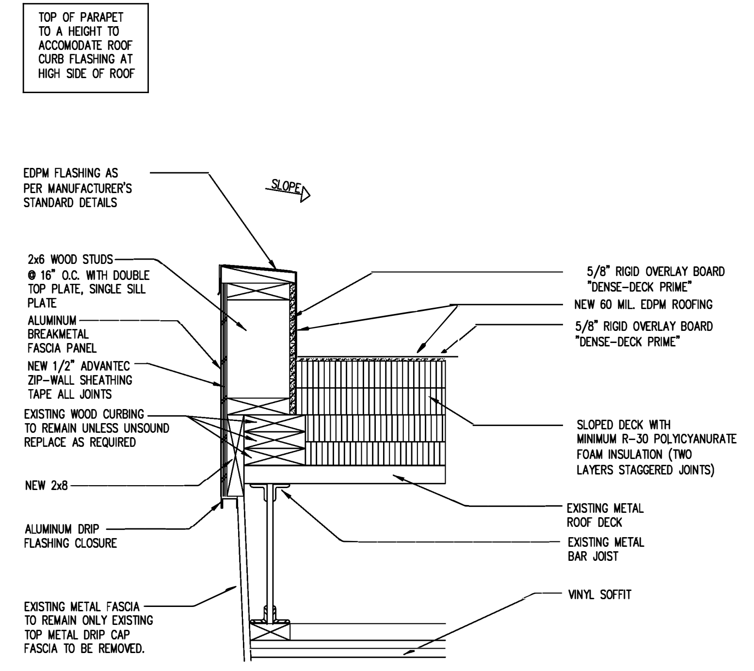
4 WALL CAP DETAIL A2 1.5"=1'-0"
