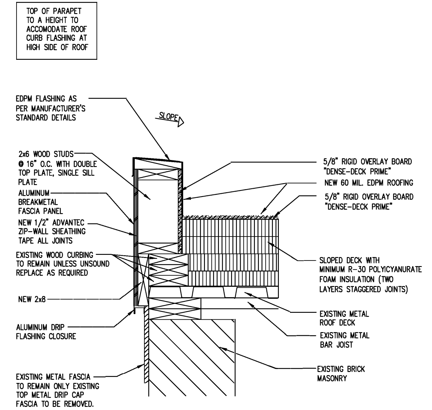
2 NON BEARING WALL CAP DETAIL A2 1.5"=1'-0"
